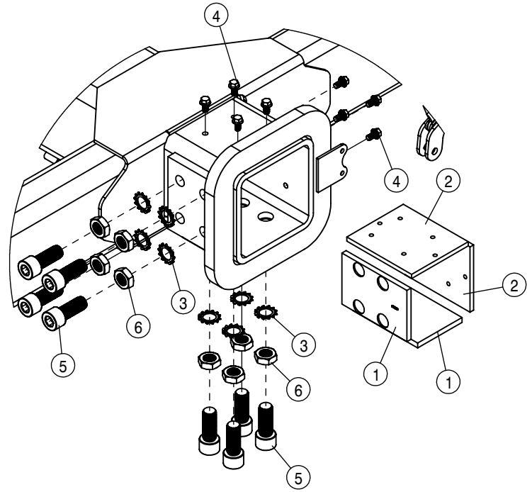
REAR MAINFRAME
