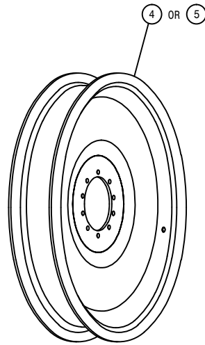
320/105 R54 RADIAL TIRE 380/90 R54 RADIAL TIRE
