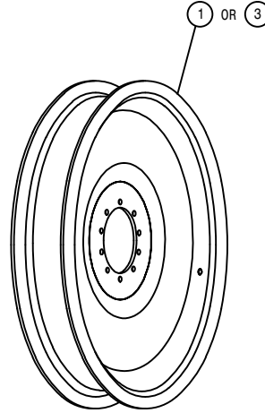
380/105 R50IF RADIAL TIRE 380/105 R50 RADIAL TIRE 320/90 R50 RADIAL TIRE
