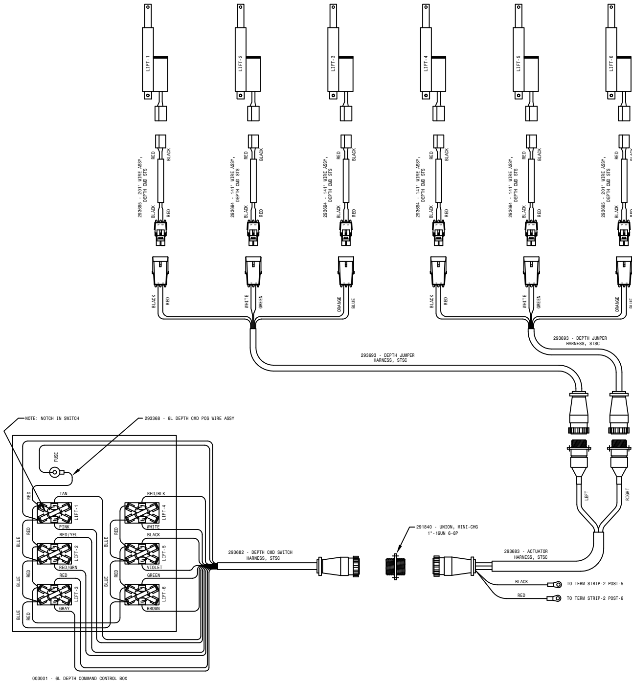
003001 - 6L DEPTH COMMAND CONTROL BOX
