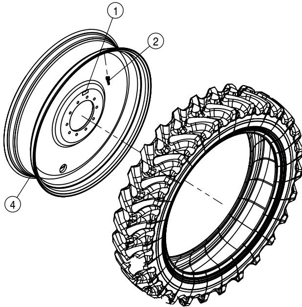
320/80 R42 RADIAL TIRE
