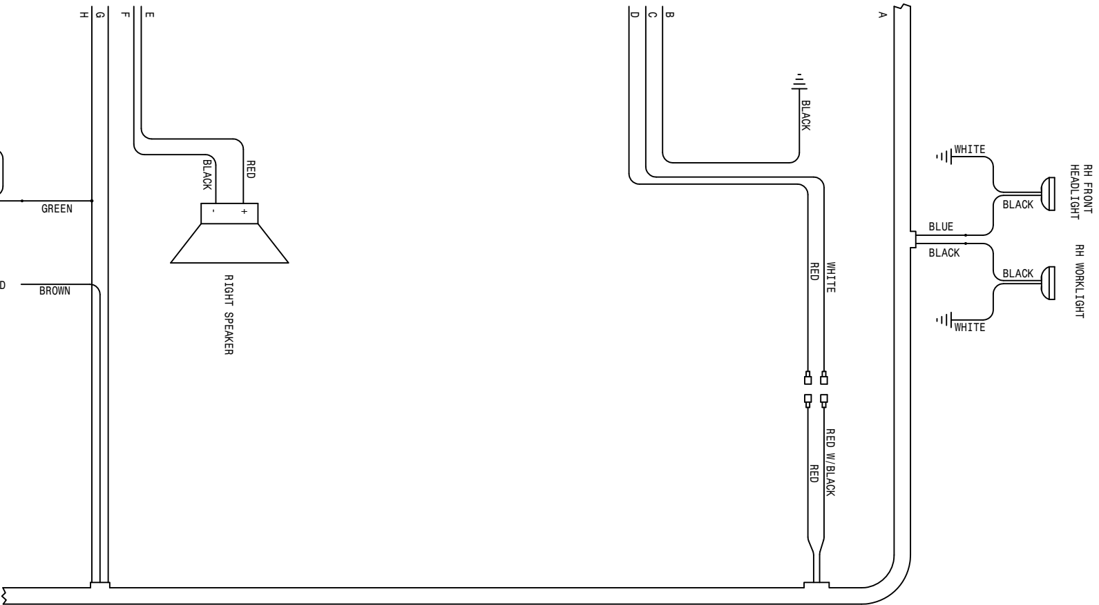
293473 - CAB WIRE HARNESS
